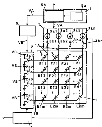
4: CONTROL UNIT 5: FIRST TEMPERATURE COMPENSATION MEANS 5a: TEMPERATURE DETECTION MEANS 5b: POWER SUPPLY CIRCUIT 6: SECOND TEMPERATURE COMPENSATION MEANS
